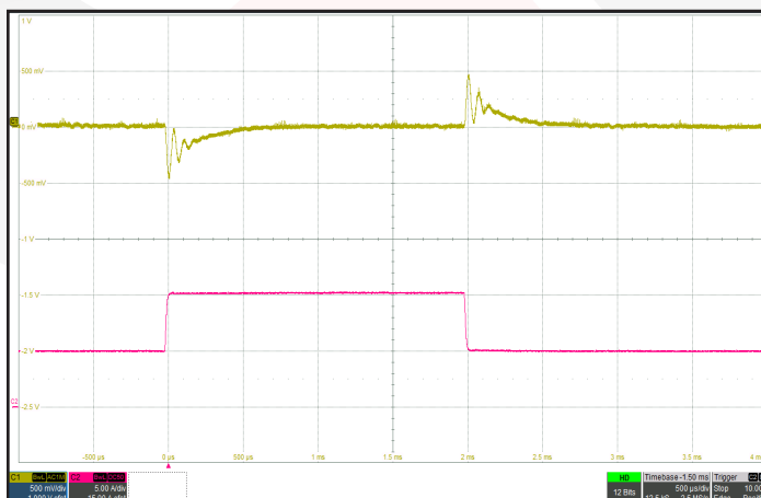
Figure 11: Output voltage response to step-change in load current 50%-100%-50% of Iout (max). No external load capacitance. Ch 1: Vout (500 mV/div). Ch 2: Iout (5 A/div). Timescale: 500µs/div.
